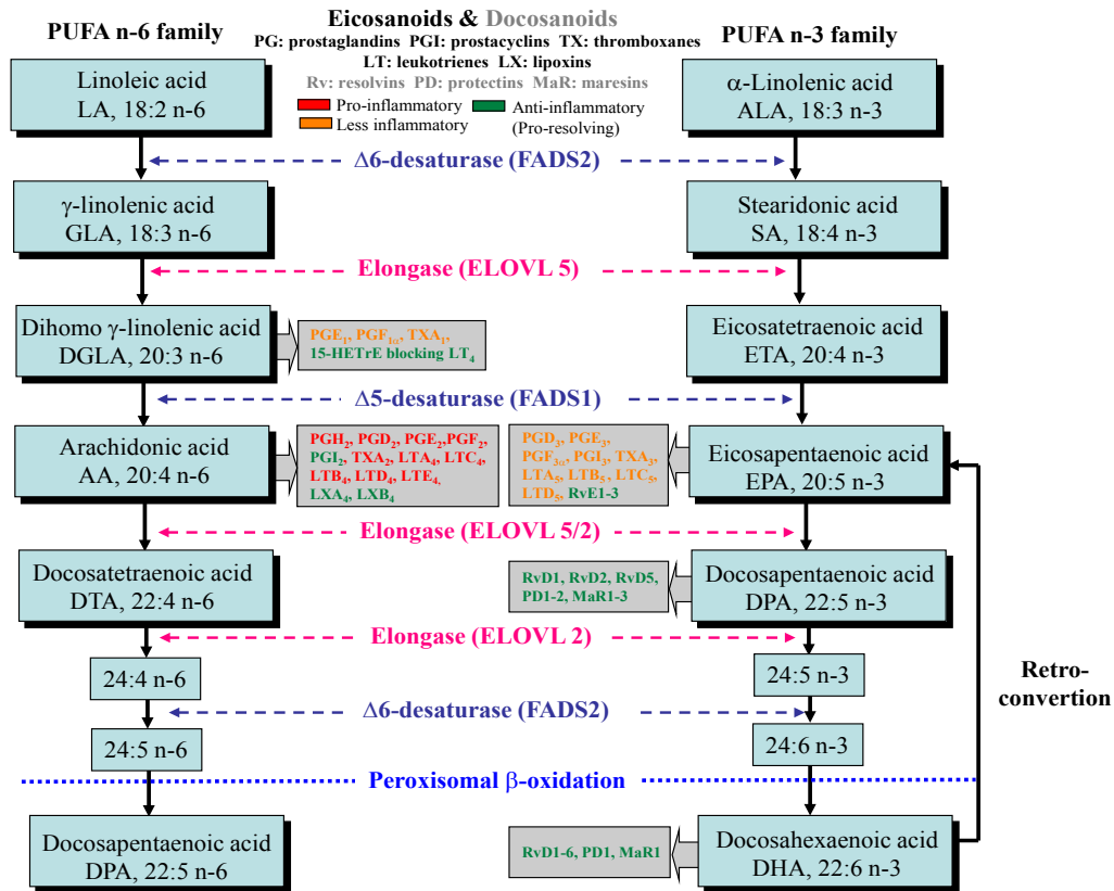
Figure 1. Schema of LC-PUFA biosynthesis in humans and related lipid mediators. ELOVL: Elongation of very long chain fatty acids genes family coding for elongases; FADS: Fatty acid desaturase genes family coding for desaturases.
